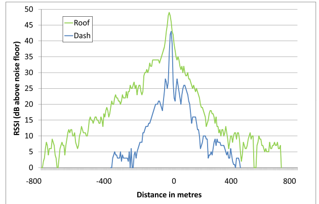
Figure 11: Effect of antenna placement on RSSI (motorway).
