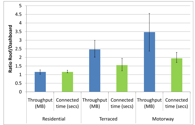
Figure 10: Effect of antenna placement.
