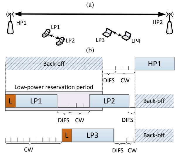
Figure 2: Illustration of the low-power reservation period (HP - high-power transmissions, LP - low-power transmissions, L - adaptive preamble): (a) network topology, (b) sample packet exchange
