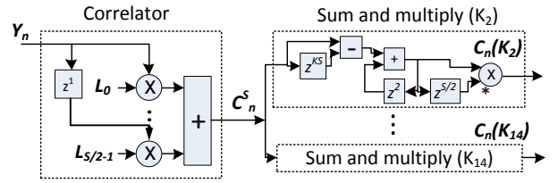
Figure 4: Adaptive detector for different preamble repetitions K = \{2, 6, 10, 14\} . Symbol z^n denotes a delay element of n cycles.
