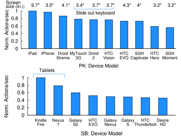
Figure 6: Normalized number of actions per unit time (maximum of 1) for different tablets phone models for PK (top) and SB (bottom). Usability in terms device type, screen size and slide out keyboards are shown.
