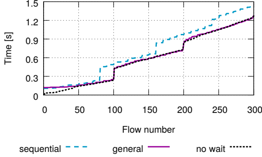
Figure 7: Flow update times with probing. There are no packet drops and the overhead of the general technique is negligible compared to the best achievable update time.
