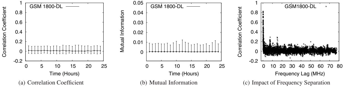
Figure 11: (a)-(b) Pair-wise correlation of GSM1800DL channels at NED across different hours of the day. Both correlation coefficient and mutual information are close to 0. (c) Correlation coefficient as a function of frequency separation. Adjacent channels are highly correlated due to imperfect alignment between measurement and service channels.
