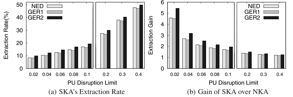
Figure 8: Impact of primary user disruption limit on spectrum extraction rate of the SKA scheme for GSM1800 DL (a) The extraction rate increases non-linearly with the disruption limit. (b) The gain of SKA over NKA decreases as we relax the primary user disruption limit.
