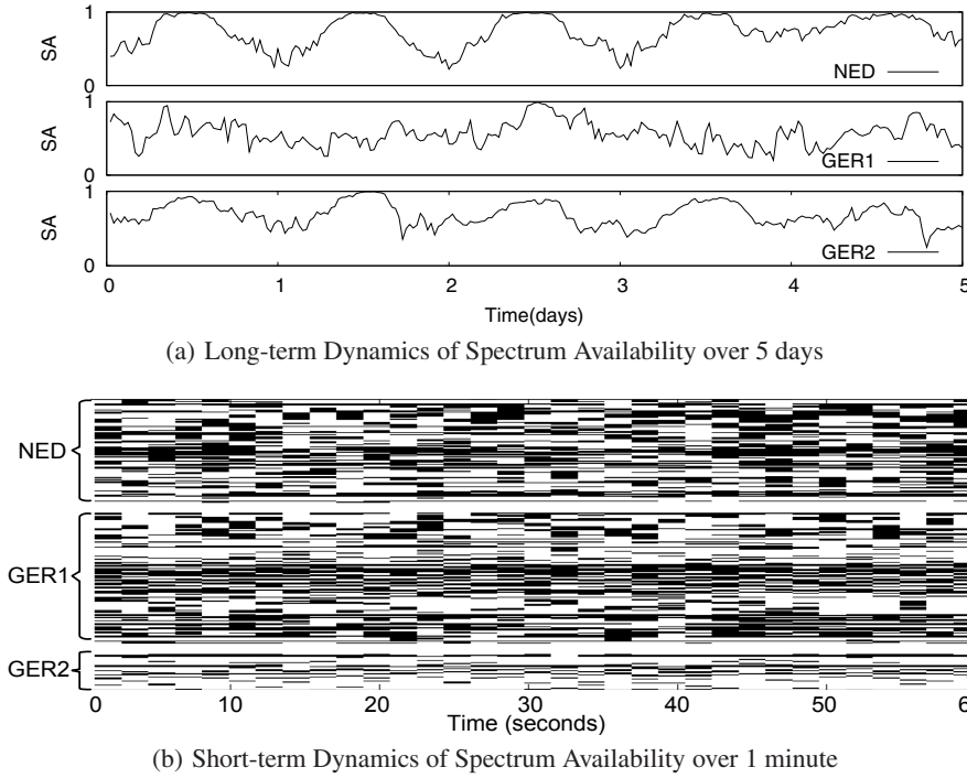
Figure 4: Long- and short-term dynamics of spectrum availability. (a) The availability (averaged over 30 minutes) varies significantly over 5 weekdays, on randomly selected GSM1800DL channels (one per location). (b) The per 1.8s availability of a 1-minute snapshot, for all the partially-used GSM1800DL channels. The availability, shown as various white strips, is scattered randomly across time.
