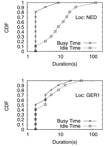
Figure 5: Cumulative distributions of channel idle and busy period on a randomly selected channel in an one hour period. Large variation in idle duration poses significant challenges for opportunistic access. The GER2 result is similar to the NED result and thus omitted.
